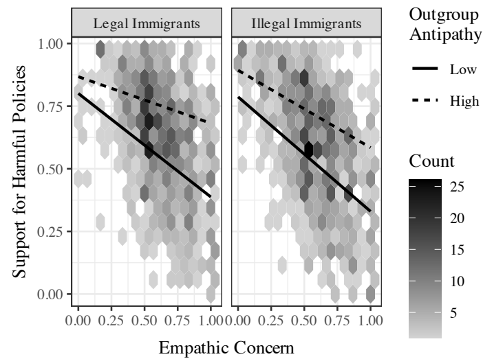
Figure H.13: Relationship between post-treatment empathic concern and post-treatment support for harmful policies, with regression lines, study 2.
