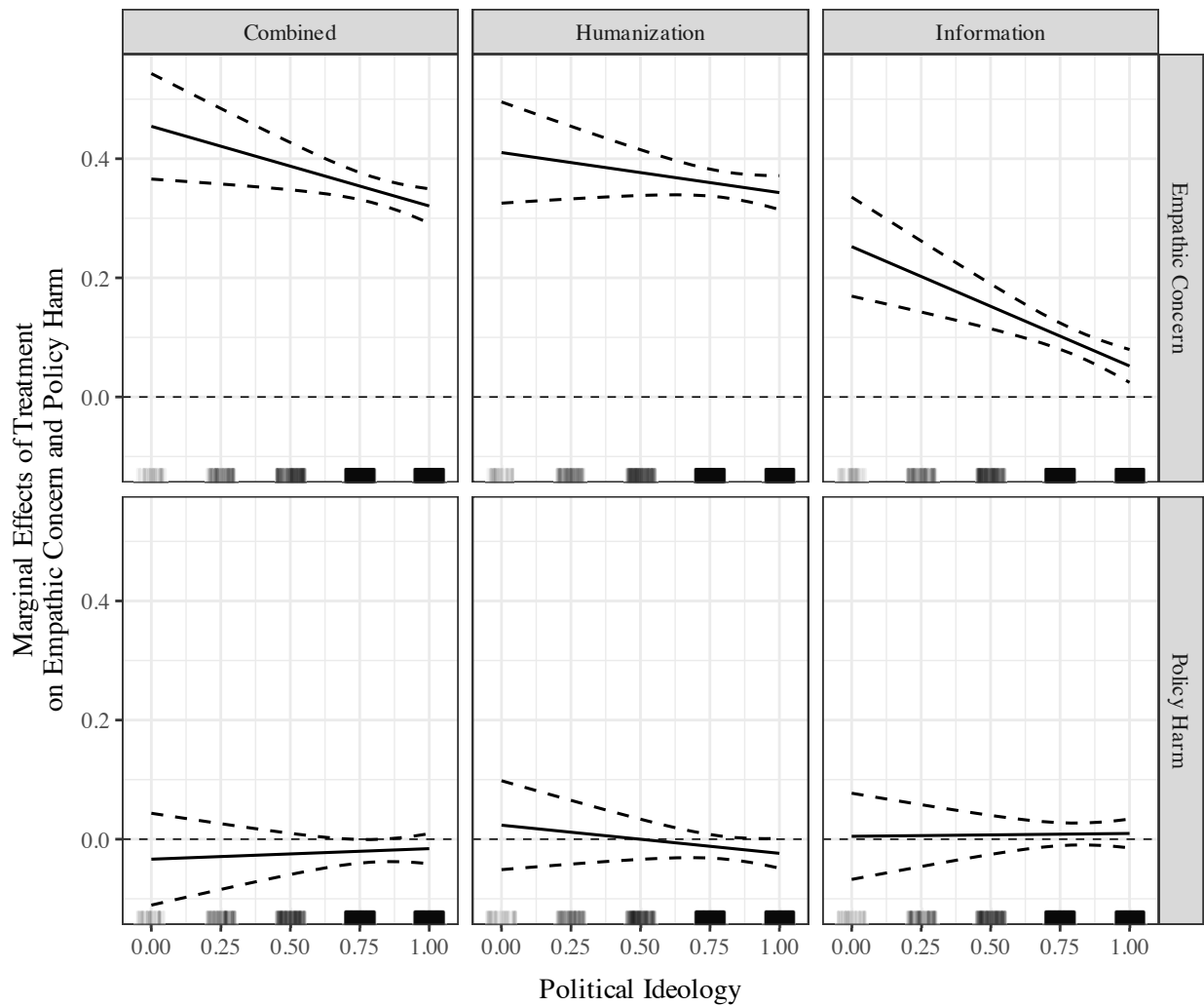
Figure H.9: Figure showing the marginal effects of the treatments on empathic concern and policy harm, by Political Ideology, for Study 1. Rug plot of Party ID included; bars represent 95% confidence intervals.
