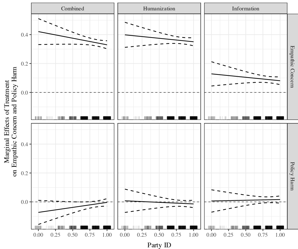
Figure H.10: Figure showing the marginal effects of the treatments on empathic concern and policy harm, by Party ID, for Study 1. Rug plot of Party ID included; bars represent 95% confidence intervals.
