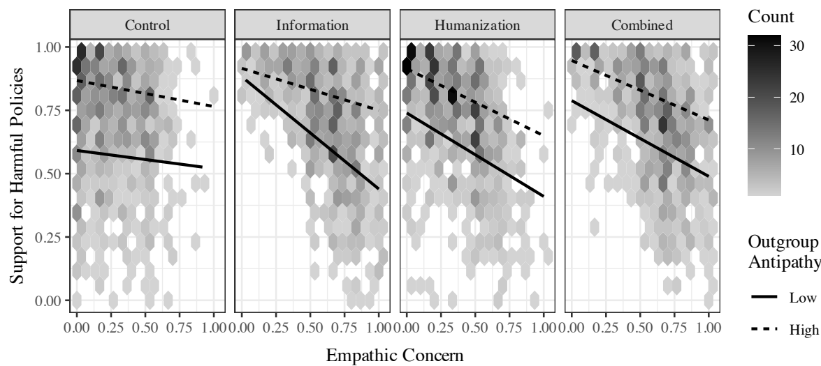
Figure H.12: Relationship between post-treatment empathic concern and post-treatment support for harmful policies, with regression lines, study 1.
