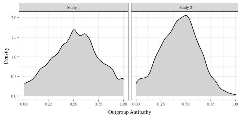
Figure B.3: Kernel density plots for Outgroup Antipathy measure, from study 1 ( n = 3,489 ) in the left panel and study 2 ( n = 1,982 ) in the right panel. Note the n -size for study 1 differs from that in the paper because of 9 respondents for whom we do not have a pre-treatment measure of outgroup antipathy.
