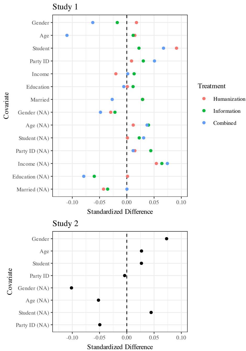
Figure E.7: Balance in Studies 1 and 2.
