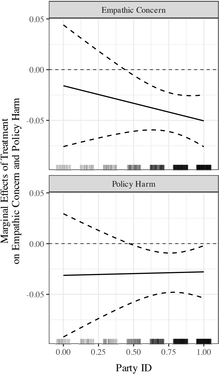
Figure H.11: Figure showing the marginal effects of the treatments on empathic concern and policy harm, by Party ID, for Study 2. Rug plot of Party ID included; bars represent 95% confidence intervals.
