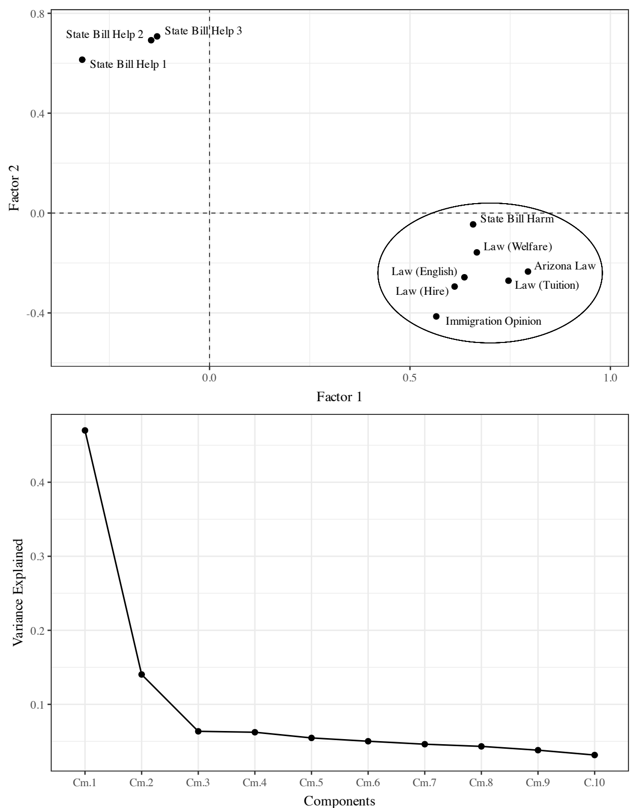
Figure D.5: Factor and Principal Components Analysis plots for 10 policy outcome measures in study 1.
