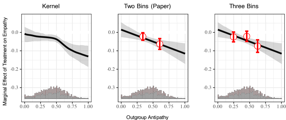
Figure H.15: Marginal effects on empathic concern from study 2, kernel estimates and tests with two and three bins
