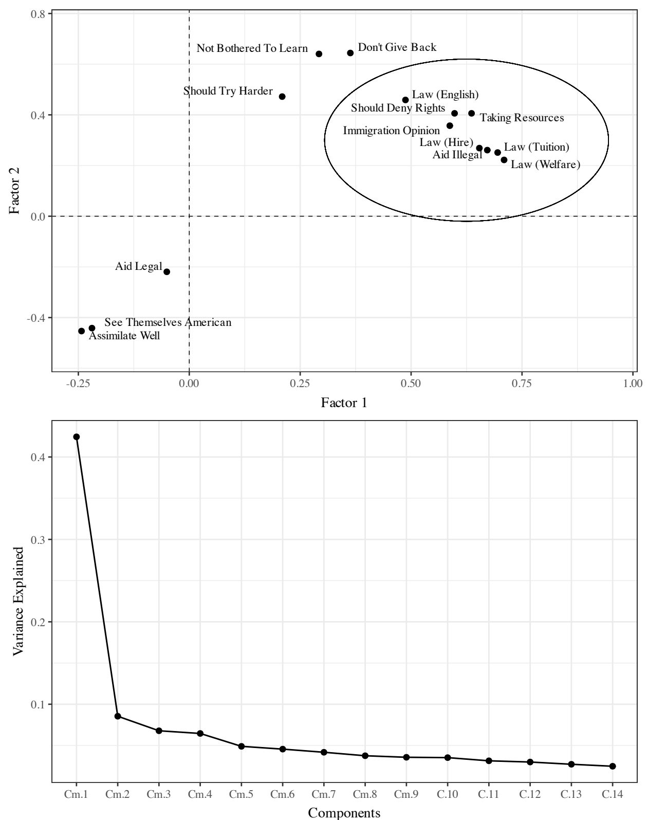
Figure D.6: Factor and Principal Components Analysis plots for 14 policy outcome measures in study 2.
