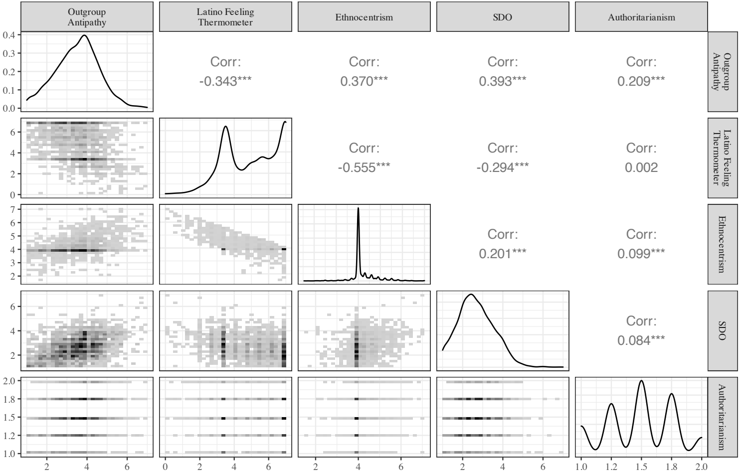
Figure C.4: Correlation Matrix and 2D Density Plots of Outgroup Antipathy and Other Common Measures.
