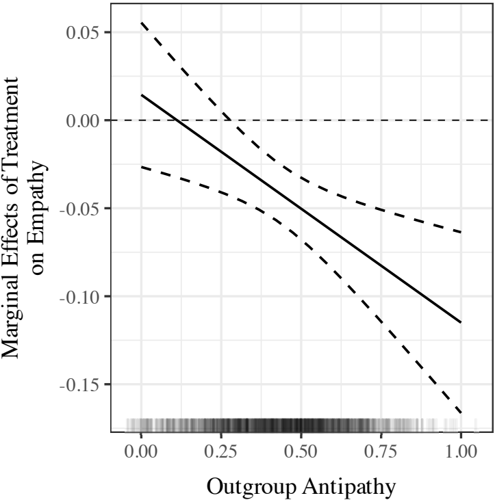
Figure H.8: Figure showing the marginal effects of the treatment on empathic Concern, by outgroup antipathy (study 2). Rug plot of outgroup antipathy included; bars represent 95% confidence intervals
