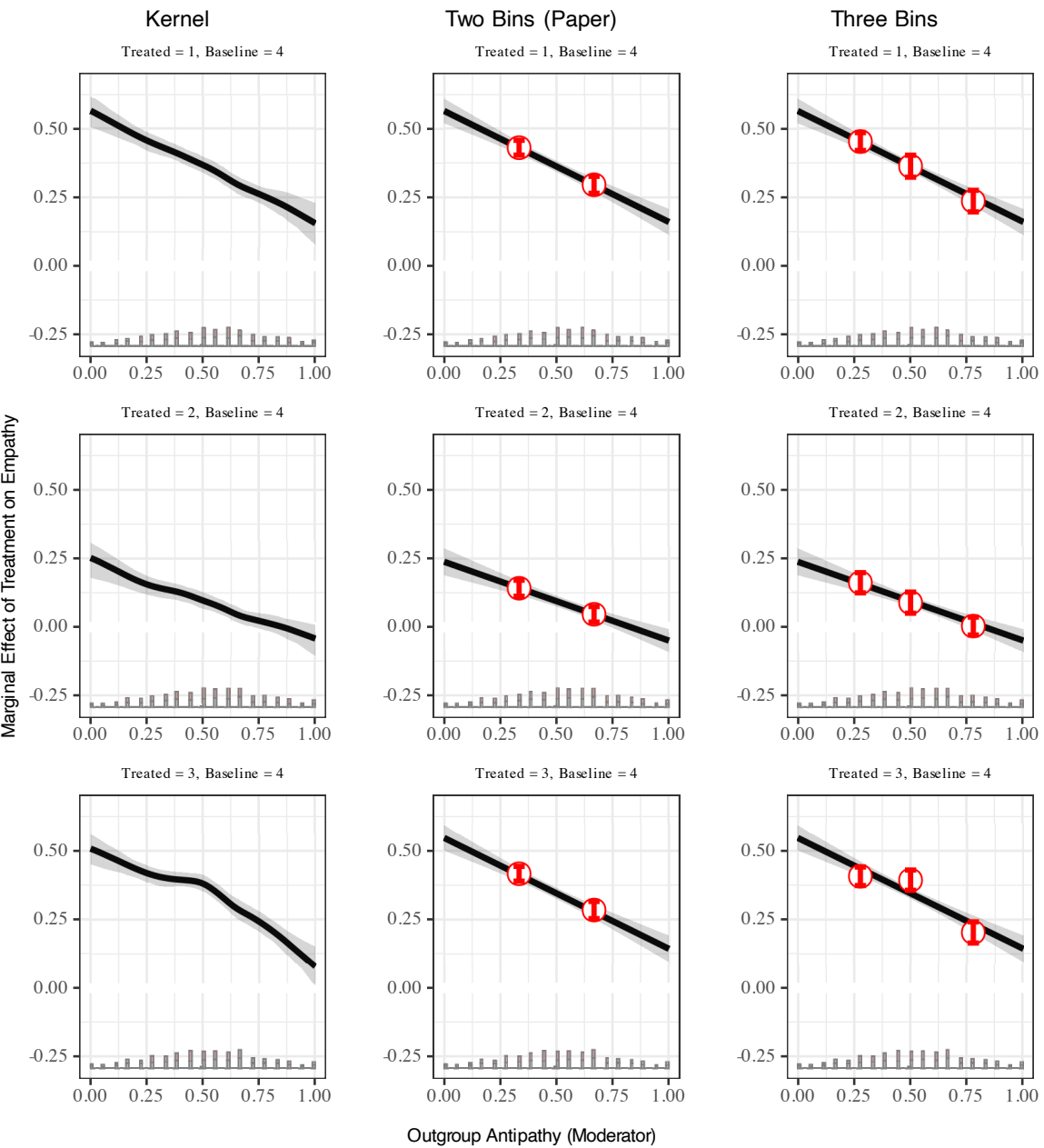
Figure H.14: Marginal effects on empathic concern from study 1, kernel estimates and tests with two and three bins
