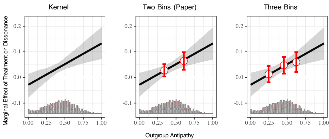
Figure H.16: Marginal effects on dissonance from study 2, kernel estimates and tests with two and three bins
